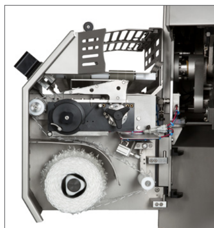
String loop feeder (BSZ 105-2)
